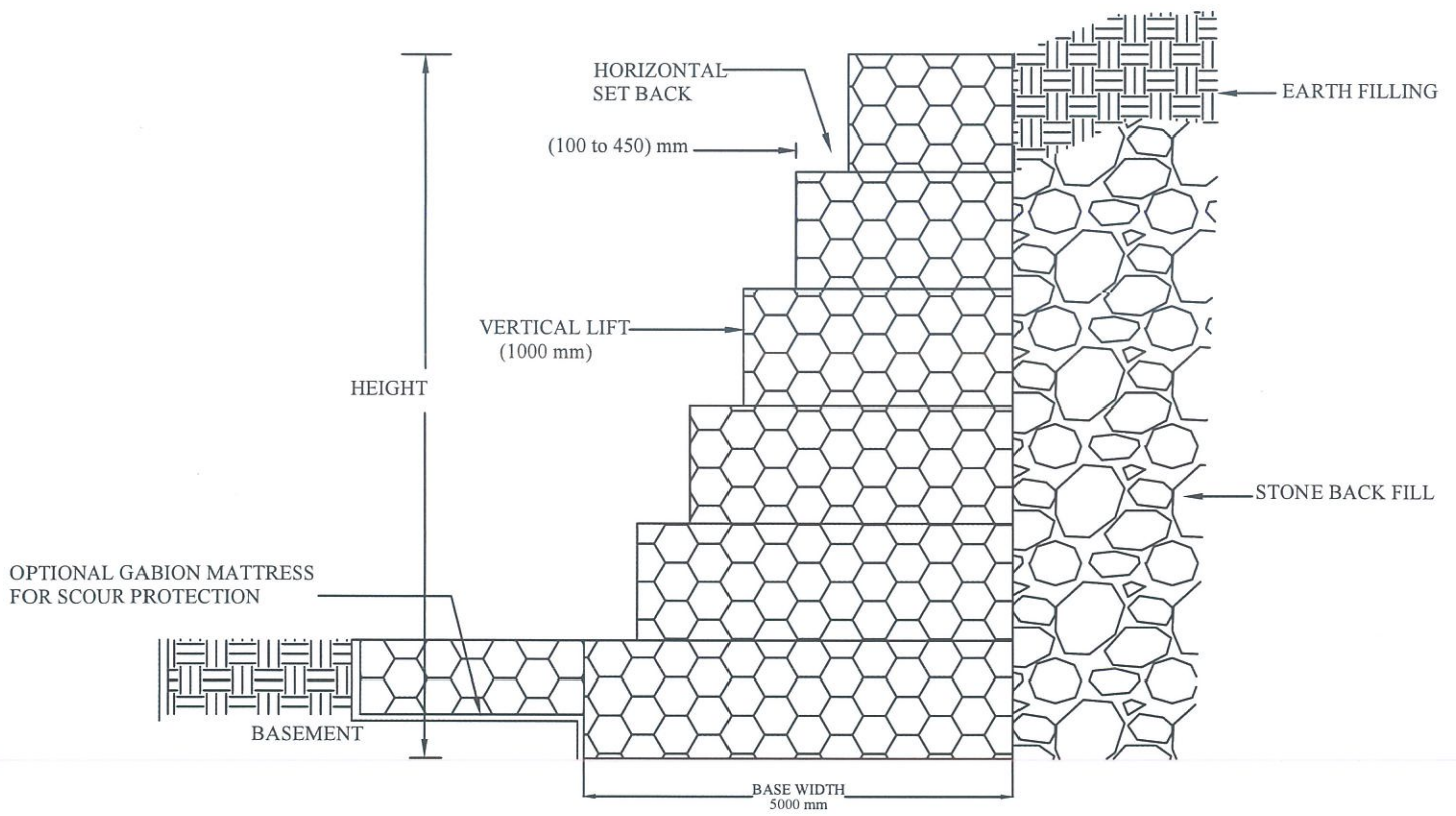
Fig:- TYPICAL DETAILS OF GABION WALL
