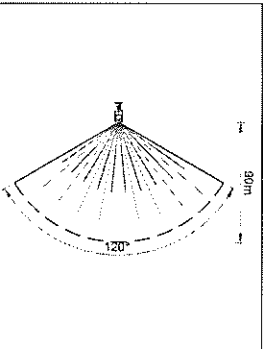
PROPOSED CCTV 1 PLAN CCTV NO. 22 (REFER TABLE NO.1 OF REPORT)
