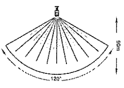
PROPOSED CCTV ANGLE CCTV NO. 28 & 29 (REFER TABLE NO. 1 OF REPORT)
